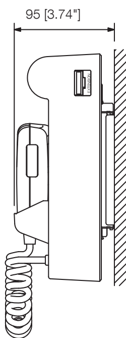
Side view with wall mounting bracket unit
