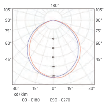
PORTAL 1x11W
