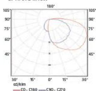
OPTIMA 2 1x40W
