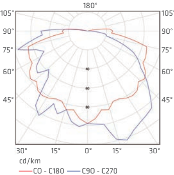
OVAL SIMETAL 1x60 W
