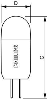
Capsule 12V 2W-20W 200lm 2700K G4 ND
